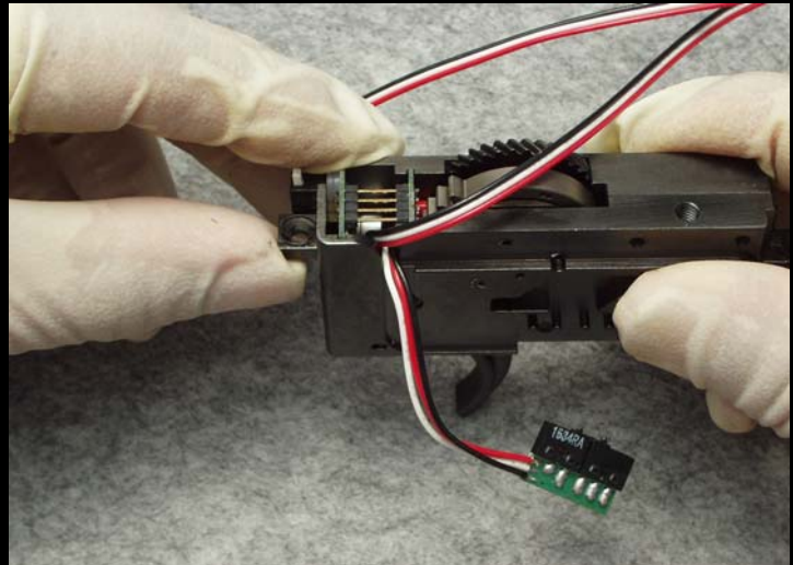
The electronic control board can be installed by your hand.
